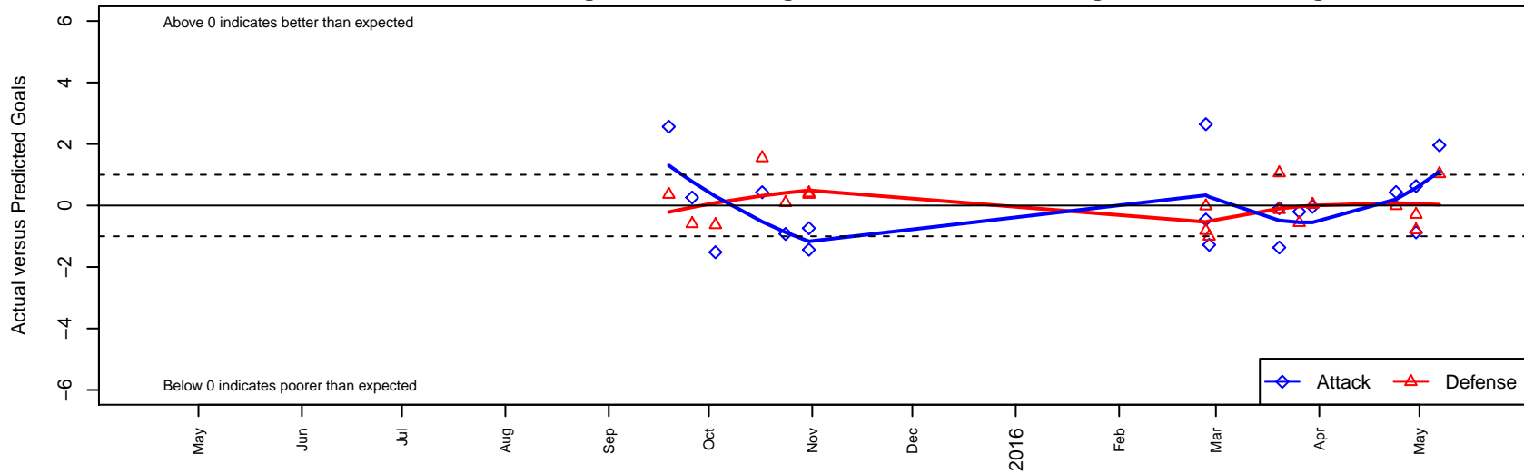
Three Rivers SC Black District G03 Dots are actual minus expected GF (blue circles) and GA (red triangles). Blue line is smoothed change in attack strength. Red is smoothed change in defense strength.
